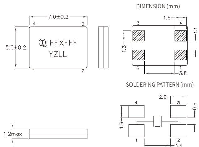
SMAC - 7050H (4 pads)
